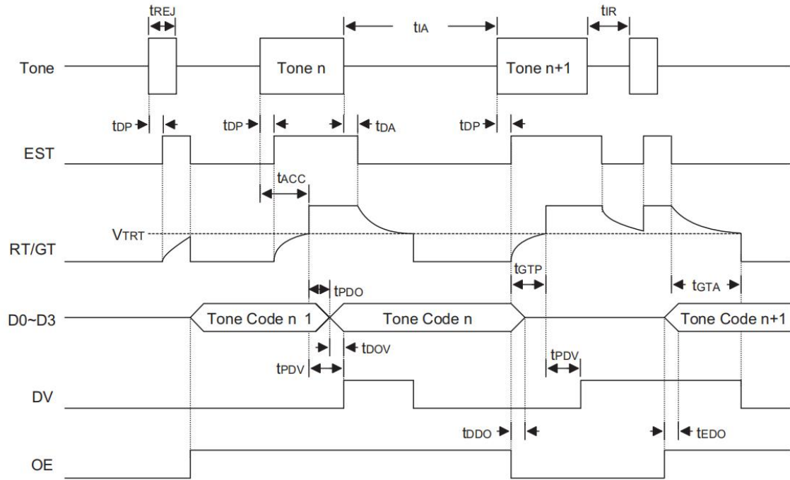
Figure 3. Steering timing
