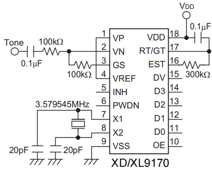
Figure 1. Test circuit
