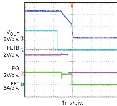
OCP Latch Mode
