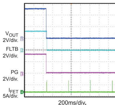
SCP Entry Retry Mode
