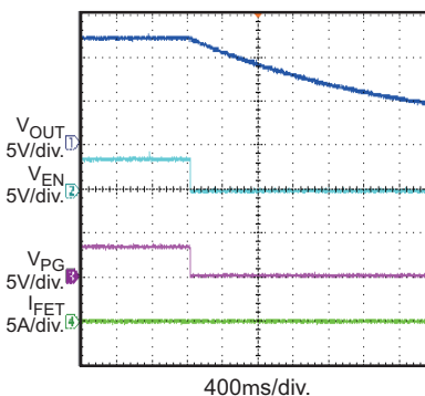
Shutdown through EN I OUT = 0A, without PD
